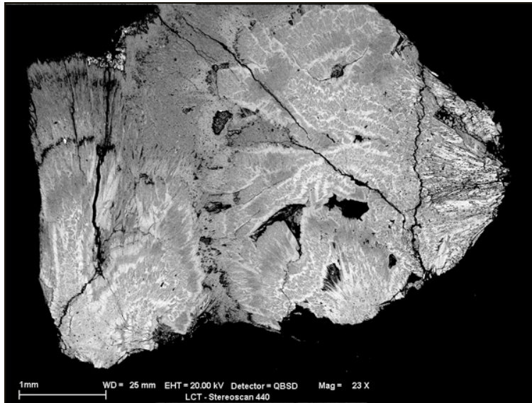
Figure 21. Back-scattered image of roscherite-group minerals from São Geraldo do Baixo. Iron oxide (white) and moraesite (dark grey) can be seen in the left part from the illustration.
