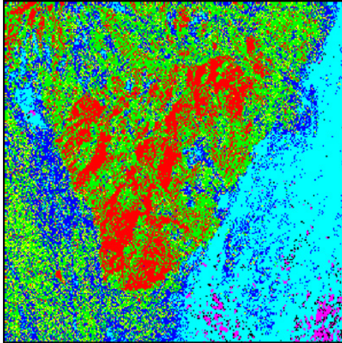
Figure 6. Digital image classification from which the geologic map was drawn, then field checked. Colors: red: chialstolite graphite hornfels; blue: quartzite; green: graphite hornfels; cyan: alluvium. Classification was accomplished using Visual_Data (Carr, 2002).
