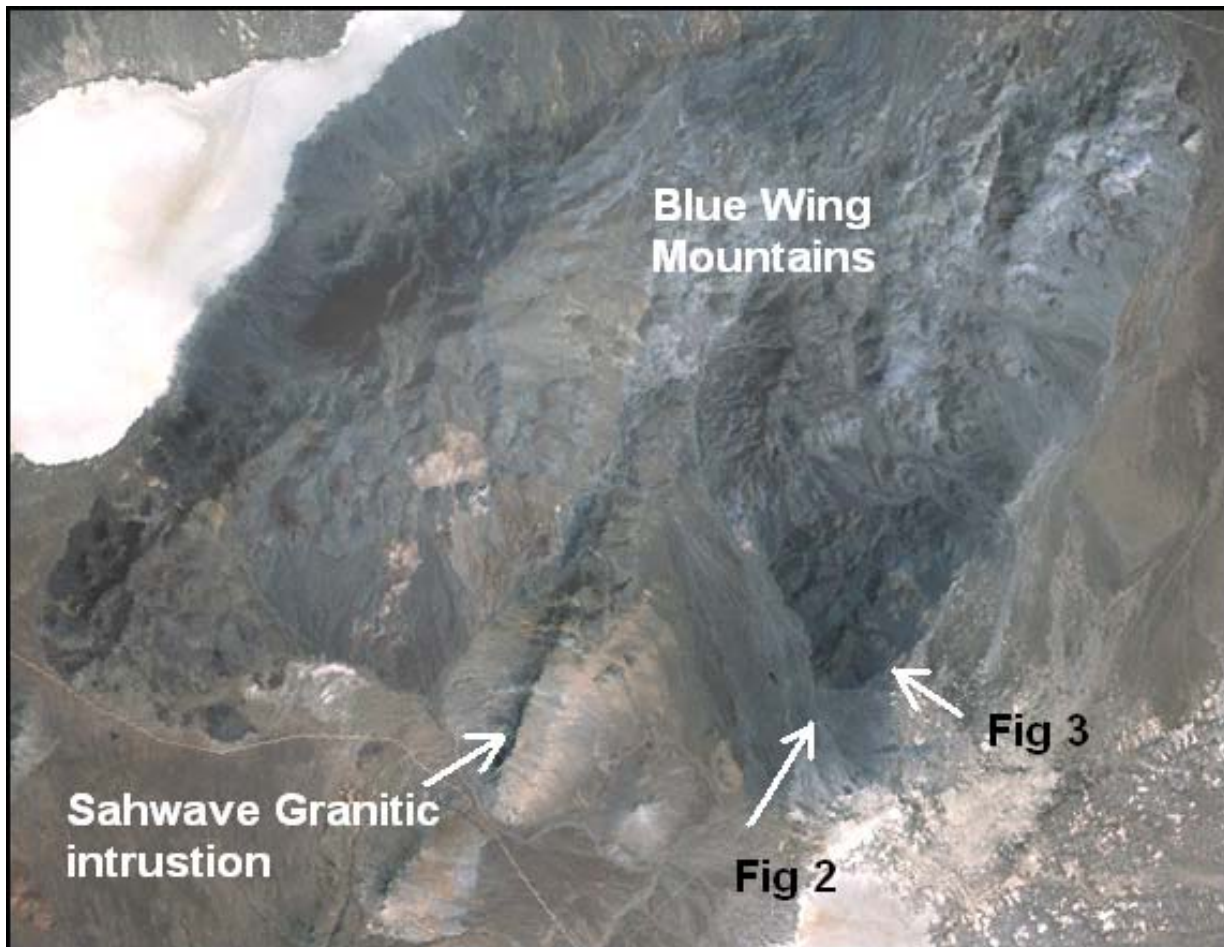
Figure 1. A true-color image composite of Landsat 7 ETM+ bands 1 (blue), 2 (green) and 3 (red); path 42 row 32; acquisition date July 27, 2000. Arrows indicate the granitic intrusion that is believed to be responsible for contact metamorphism and look directions for the digital photos shown in Figures 2 and 3. Satellite image data was obtained from the University of Maryland, Global Land Cover Facility ( http://glcf.umd.edu/data/landsat/ ). Assembly into a true-color composite was accomplished using Visual_Data (Carr, 2002).
