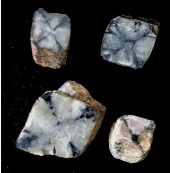
Figure 8. Four polished cross-sections showing a variety of forms and colors exhibited by typical crystals from the Blue Wing Mountains. The upper-right cross-section shows the iridescence imparted to the crystal by its partial alteration to sericite. The lower-left crystal is 2 cm on edge. Collection and photo: James Carr.
