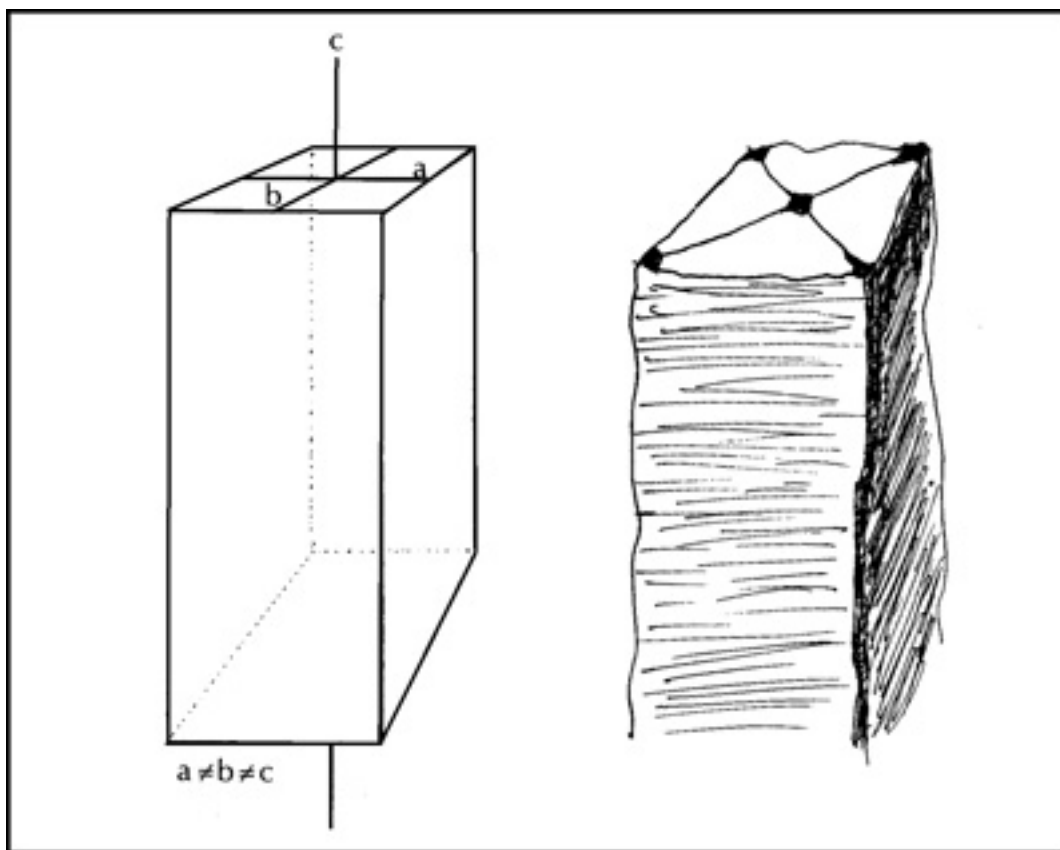
Figure 7. A sketch of the ideal orthorhombic crystal geometry (left) compared with the actual rough chialitolite crystal (right). The right-hand sketch is typical of the crystals found in the Blue Wing Mountains. James Carr drawings.
