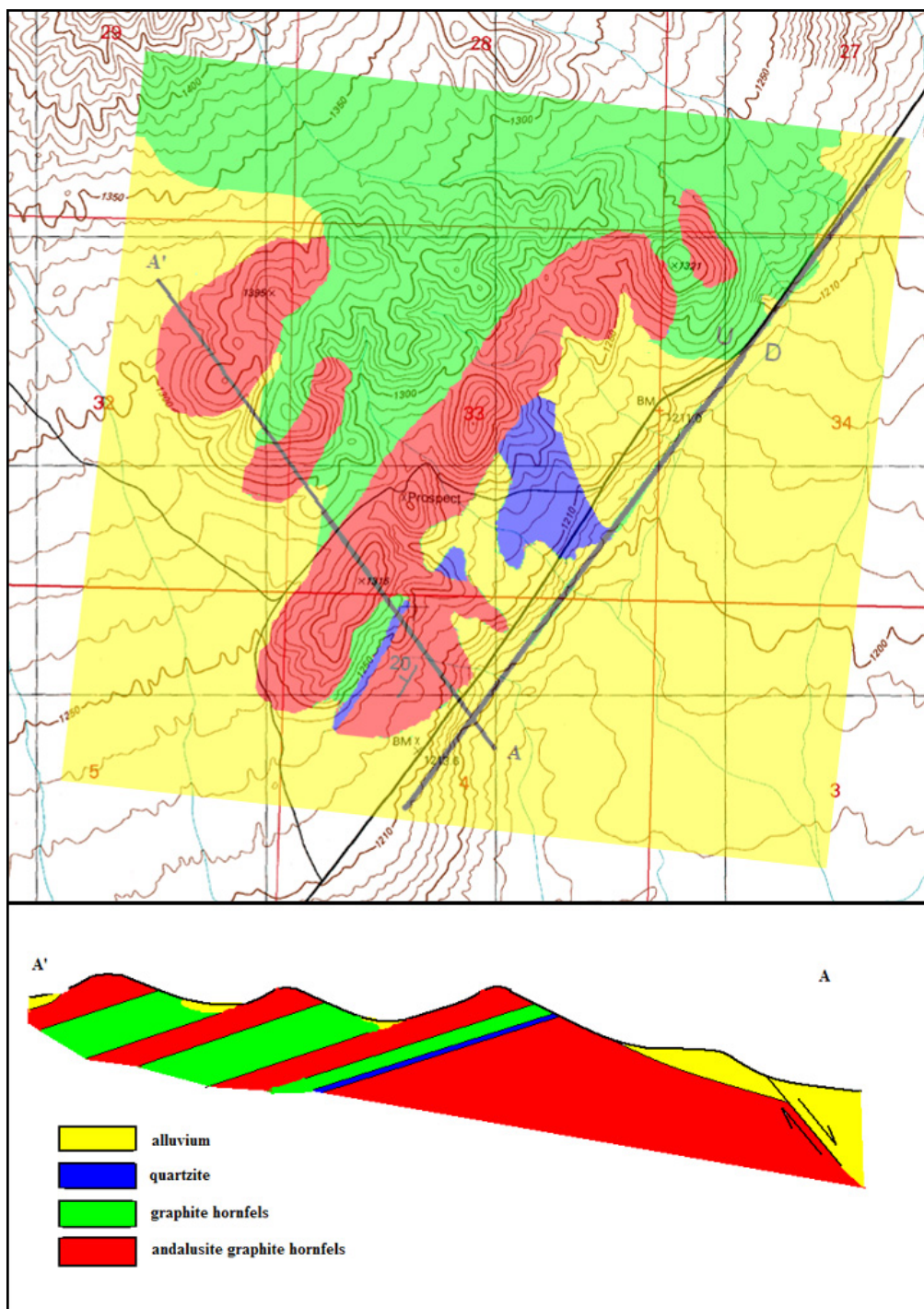
Figure 5. Geologic map of the southeastern portion of the Blue Wing Mountains. Units shown are: Red: andalusite (chiasolite) graphite hornfels; Blue: quartzite; Green: graphite hornfels; Yellow: alluvium and playa sediments. This map was created using Landsat 7 images fused to 15 m spatial resolution, classified then field checked. Adobe Photoshop 8.0 was used to overlay the geologic map on a digital image of the USGS 7.5 quadrangle maps, Juniper Pass and Blue Wing Flat quads. The line, A to A', locates the cross-section displayed in the cross-section ( below ) showing beds dipping 20 degrees to the northwest.
